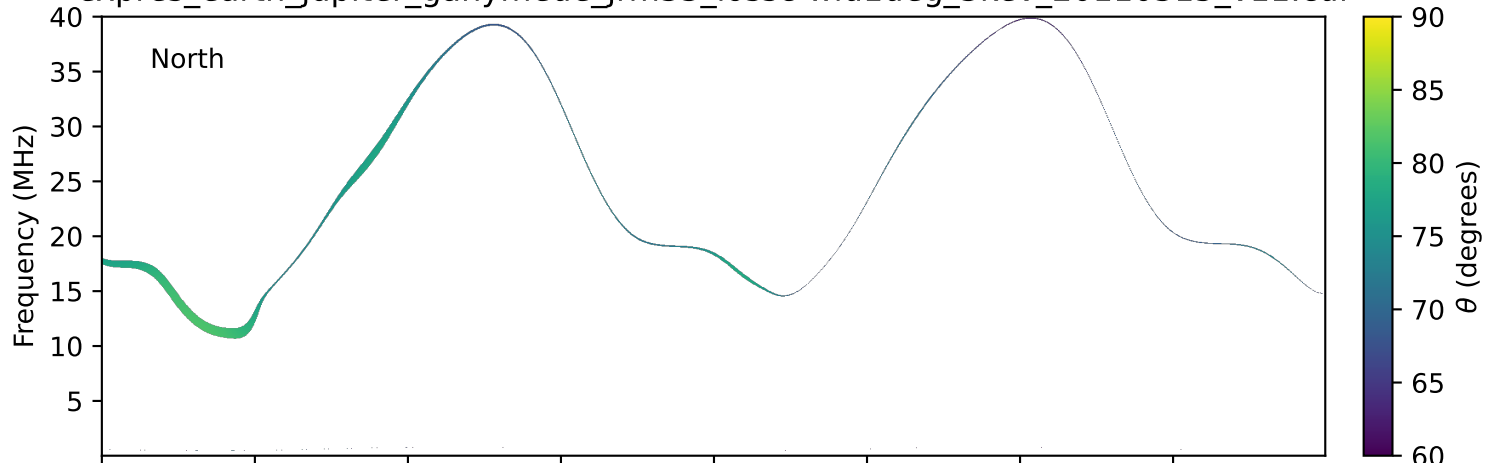
expres_earth_jupiter_ganymede_jrm33_lossc-wid1deg_3kev_20110315_v11.cdf
