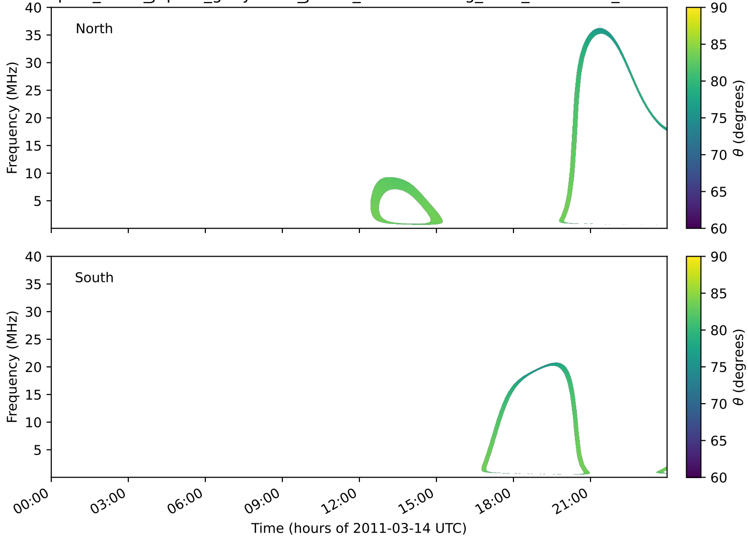
expres_earth_jupiter_ganymede_jrm33_lossc-wid1deg_3kev_20110314_v11.cdf
