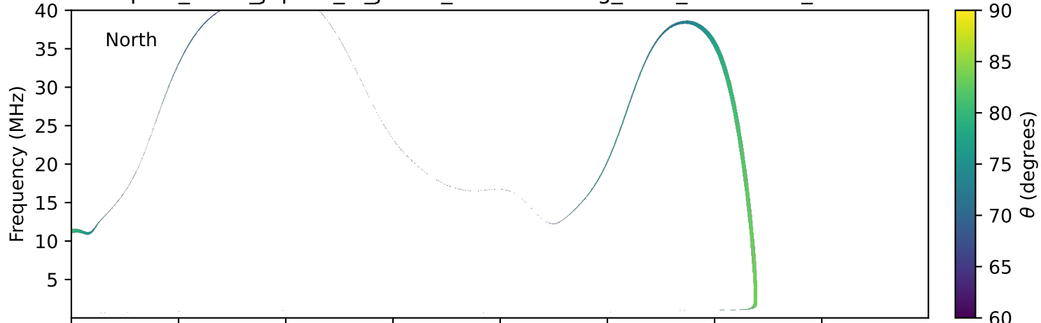
expres_earth_jupiter_io_jrm33_lossc-wid1deg_3kev_20110222_v11.cdf
