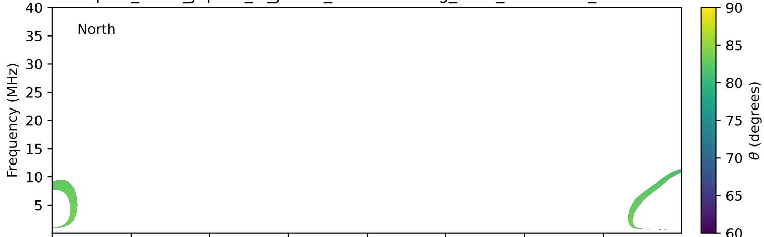
expres_earth_jupiter_io_jrm33_lossc-wid1deg_3kev_20110221_v11.cdf
