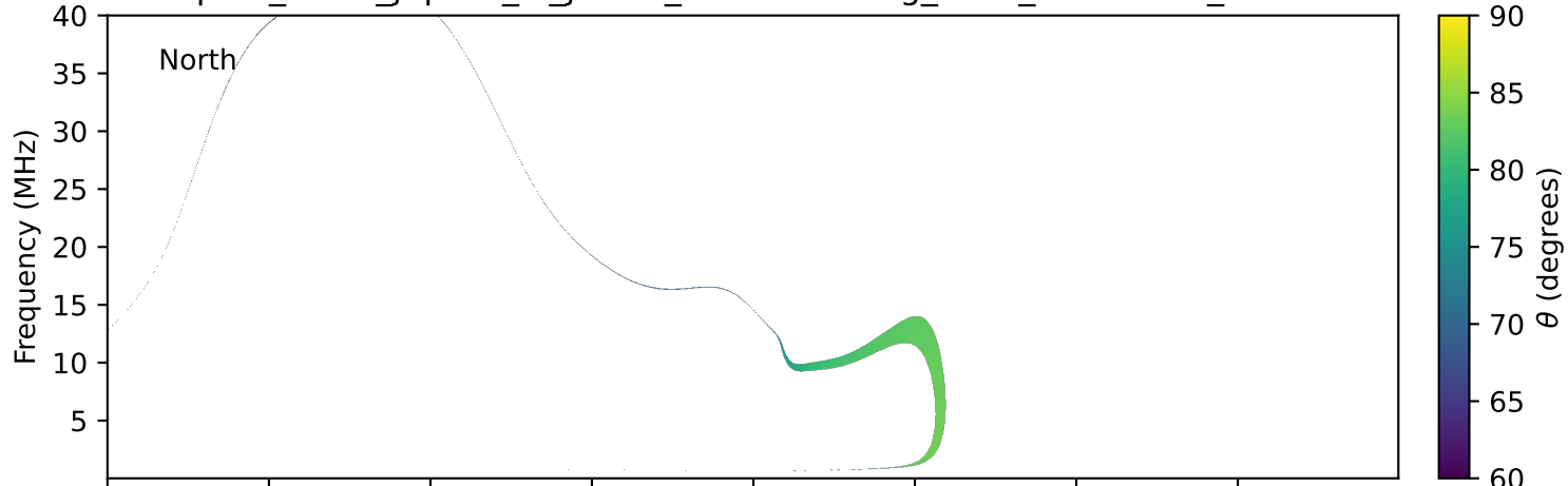
expres_earth_jupiter_io_jrm33_lossc-wid1deg_3kev_20110208_v11.cdf
