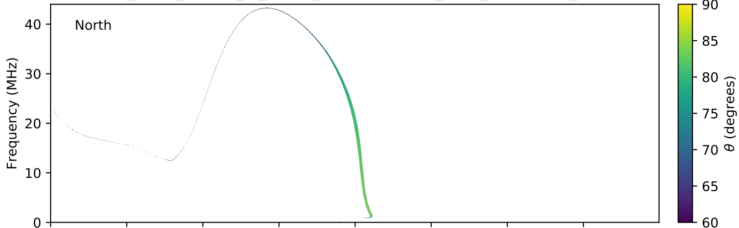
expres_earth_jupiter_io_jrm09_lossc-wid1deg_3kev_20110224_v01.cdf
