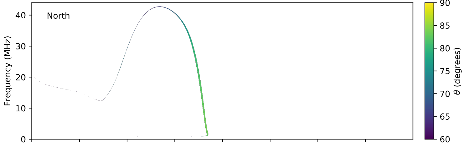
expres_earth_jupiter_io_jrm09_lossc-wid1deg_3kev_20110217_v01.cdf
