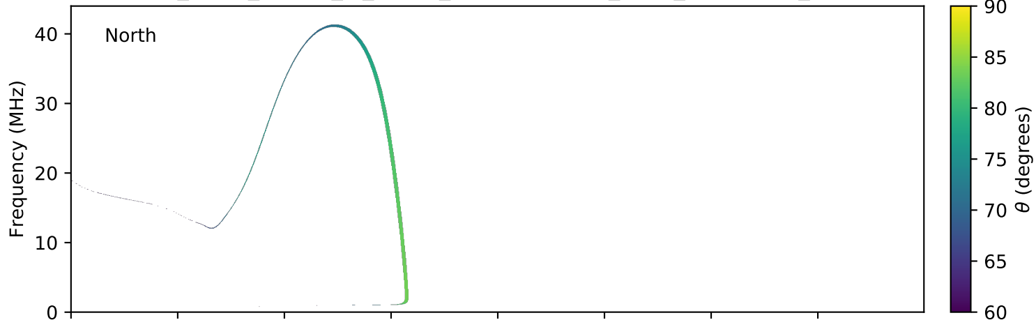
expres_earth_jupiter_io_jrm09_lossc-wid1deg_3kev_20110210_v01.cdf
