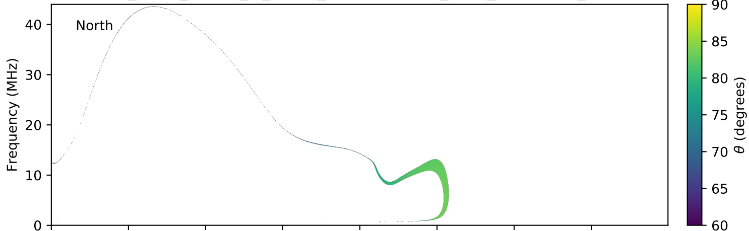
expres_earth_jupiter_io_jrm09_lossc-wid1deg_3kev_20110208_v01.cdf
