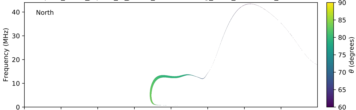
expres_earth_jupiter_io_jrm09_lossc-wid1deg_3kev_20110202_v01.cdf
