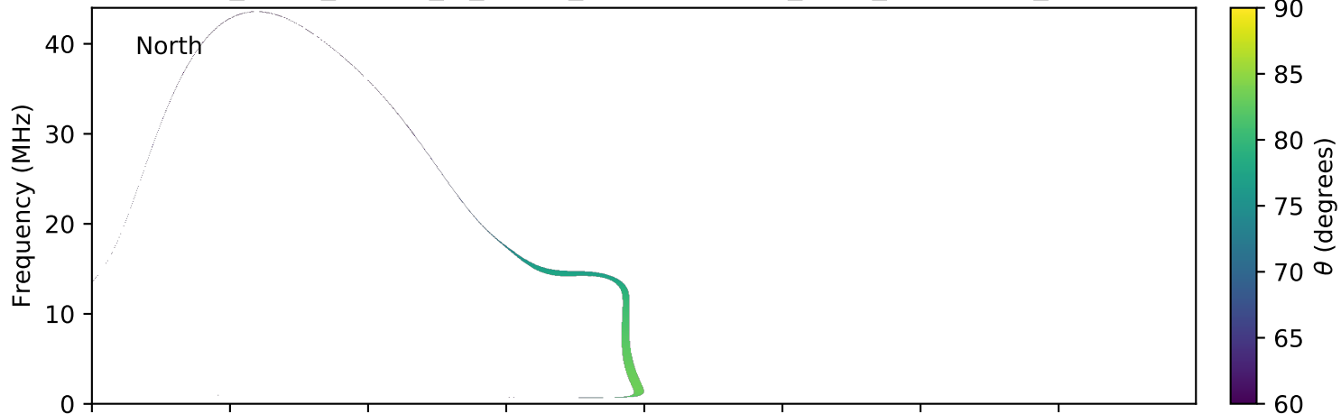
expres_earth_jupiter_io_jrm09_lossc-wid1deg_3kev_20110201_v01.cdf
