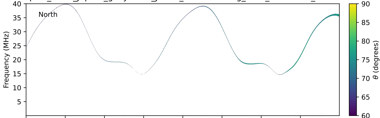
expres_earth_jupiter_ganymede_jrm33_lossc-wid1deg_3kev_20110223_v11.cdf
