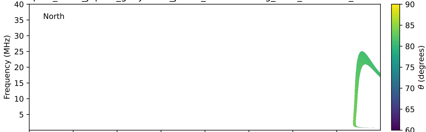
expres_earth_jupiter_ganymede_jrm33_lossc-wid1deg_3kev_20110213_v11.cdf
