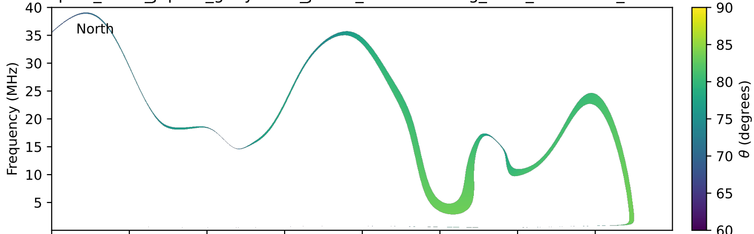
expres_earth_jupiter_ganymede_jrm33_lossc-wid1deg_3kev_20110202_v11.cdf
