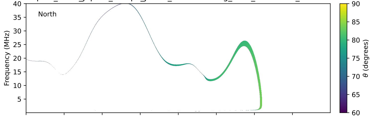
expres_earth_jupiter_europa_jrm33_lossc-wid1deg_3kev_20110222_v11.cdf
