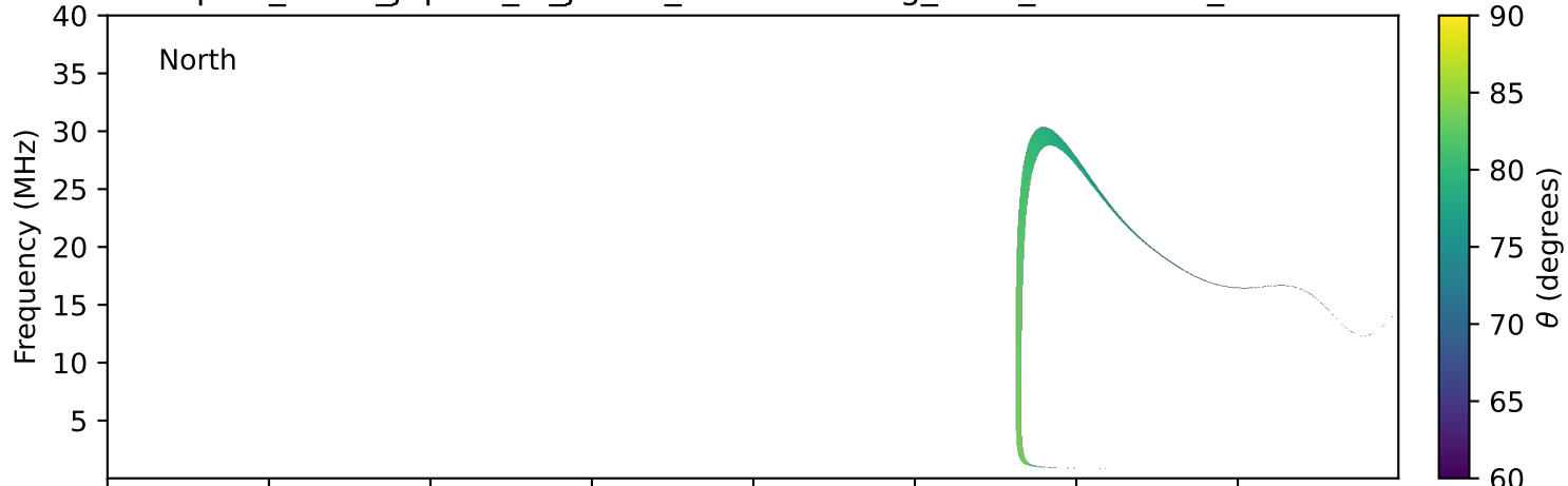
expres_earth_jupiter_io_jrm33_lossc-wid1deg_3kev_20110131_v11.cdf
