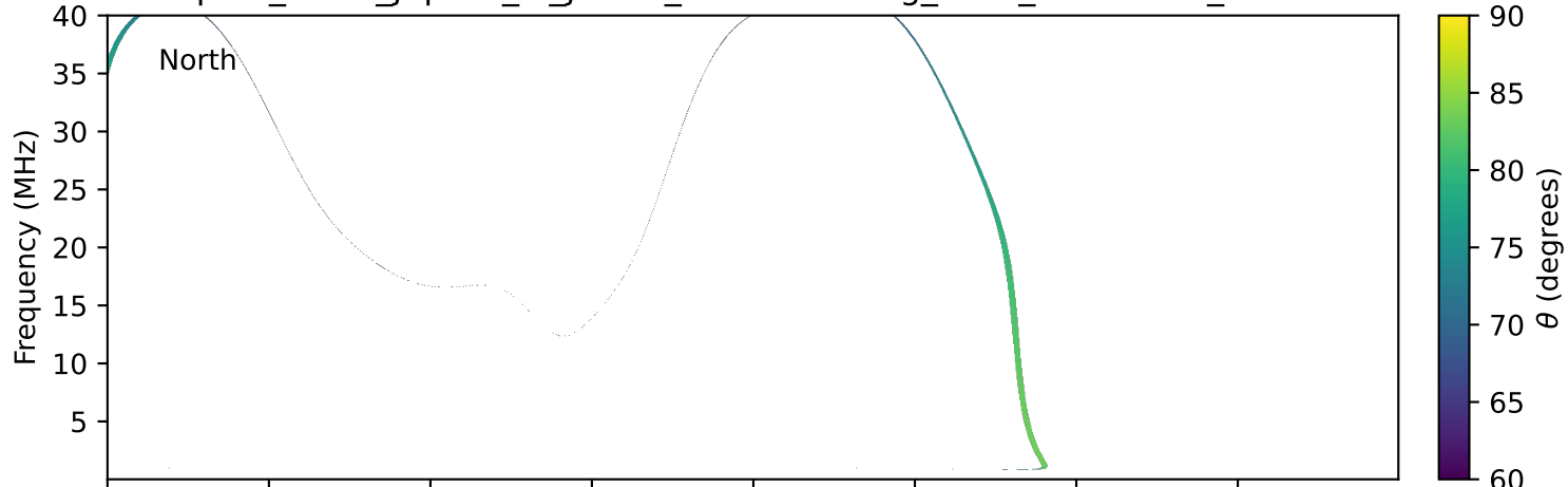
expres_earth_jupiter_io_jrm33_lossc-wid1deg_3kev_20110130_v11.cdf
