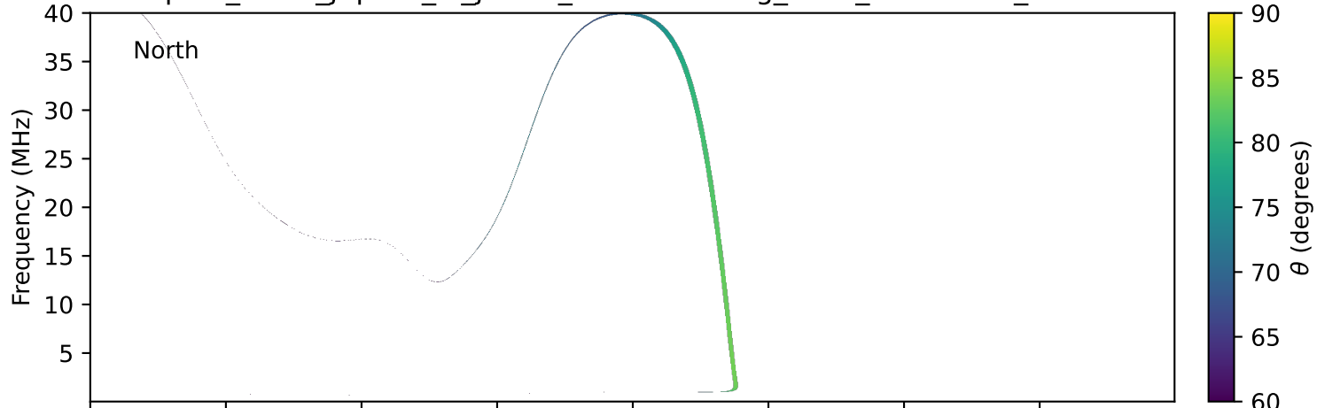
expres_earth_jupiter_io_jrm33_lossc-wid1deg_3kev_20110116_v11.cdf
