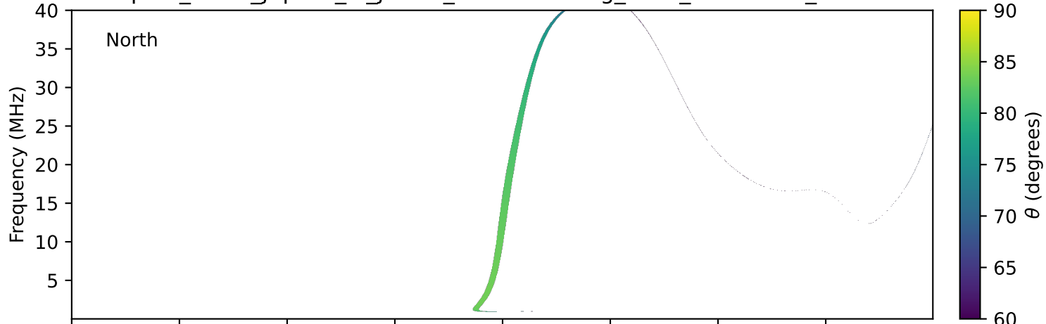
expres_earth_jupiter_io_jrm33_lossc-wid1deg_3kev_20110110_v11.cdf
