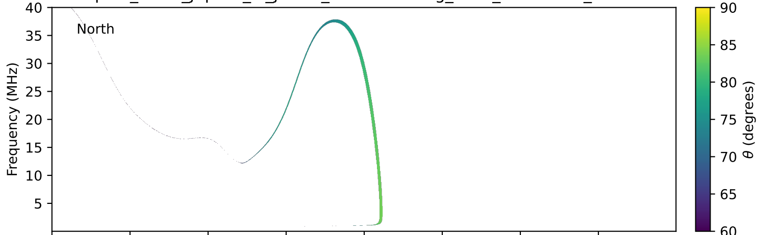
expres_earth_jupiter_io_jrm33_lossc-wid1deg_3kev_20110109_v11.cdf
