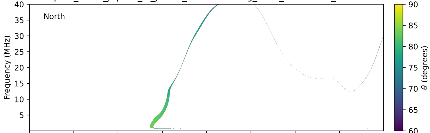
expres_earth_jupiter_io_jrm33_lossc-wid1deg_3kev_20110103_v11.cdf
