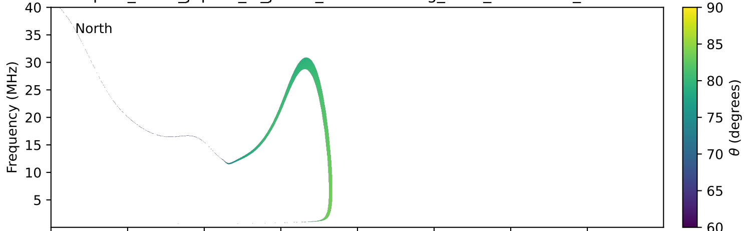
expres_earth_jupiter_io_jrm33_lossc-wid1deg_3kev_20110102_v11.cdf
