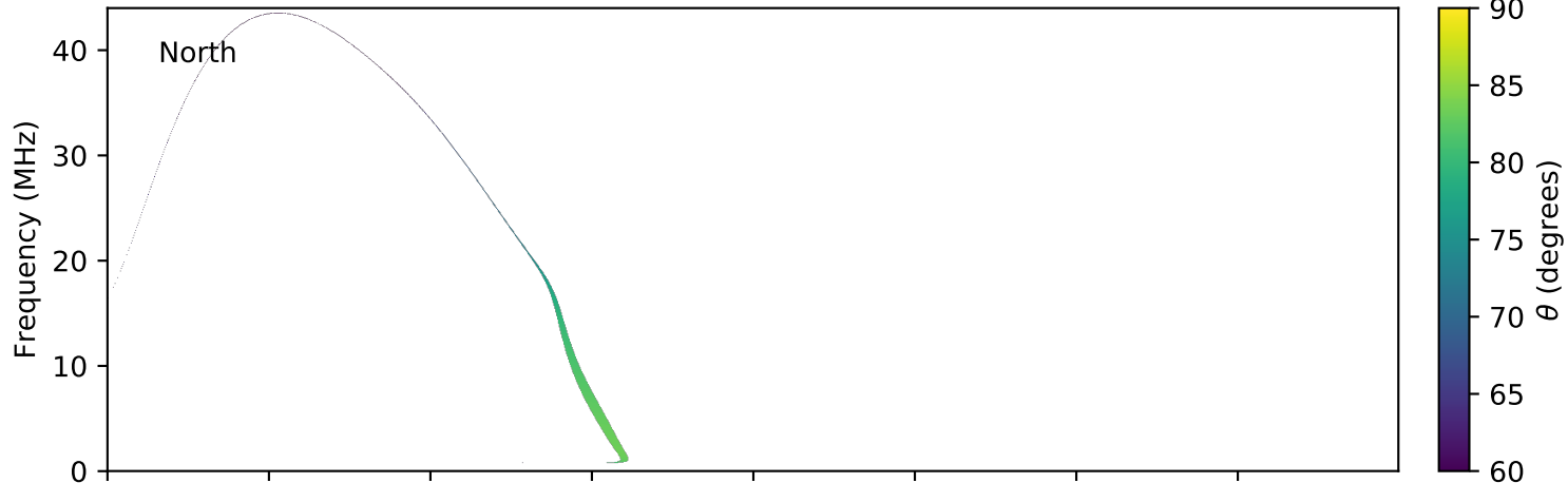
expres_earth_jupiter_io_jrm09_lossc-wid1deg_3kev_20110125_v01.cdf
