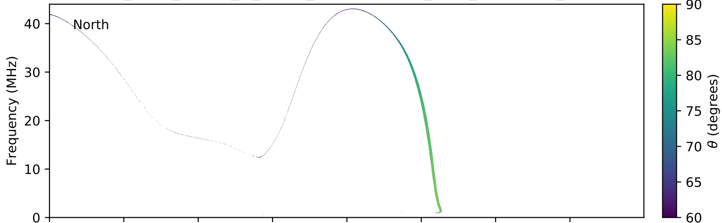
expres_earth_jupiter_io_jrm09_lossc-wid1deg_3kev_20110123_v01.cdf
