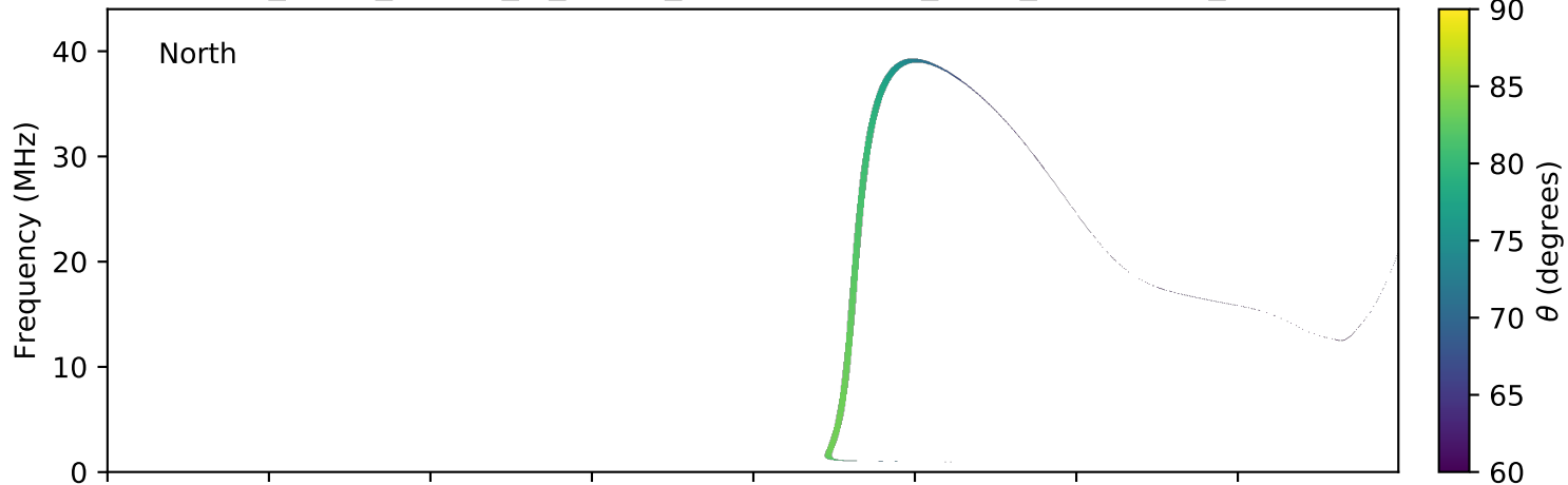
expres_earth_jupiter_io_jrm09_lossc-wid1deg_3kev_20110117_v01.cdf
