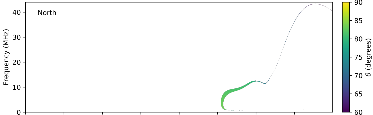
expres_earth_jupiter_io_jrm09_lossc-wid1deg_3kev_20110108_v01.cdf
