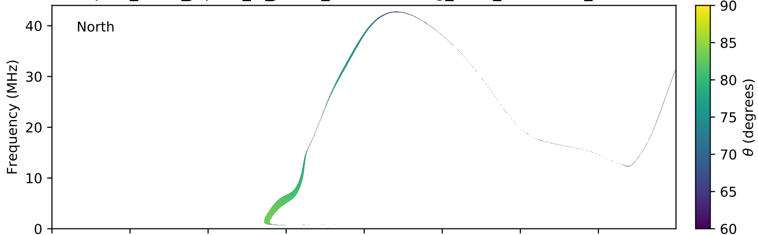
expres_earth_jupiter_io_jrm09_lossc-wid1deg_3kev_20110103_v01.cdf
