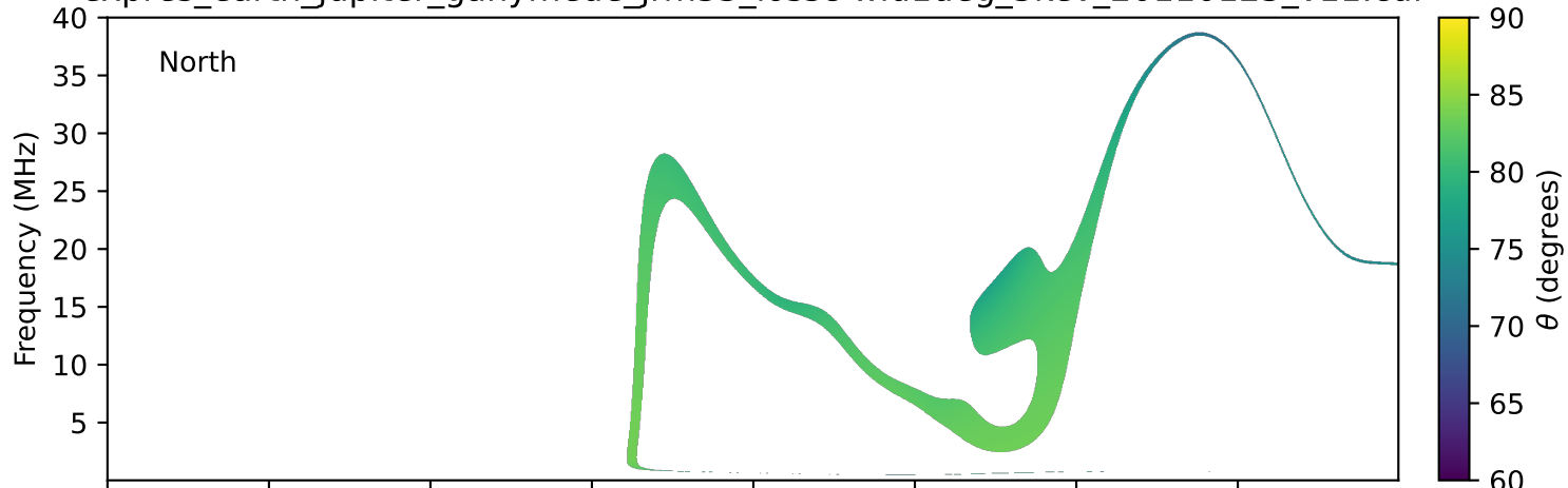
expres_earth_jupiter_ganymede_jrm33_lossc-wid1deg_3kev_20110123_v11.cdf
