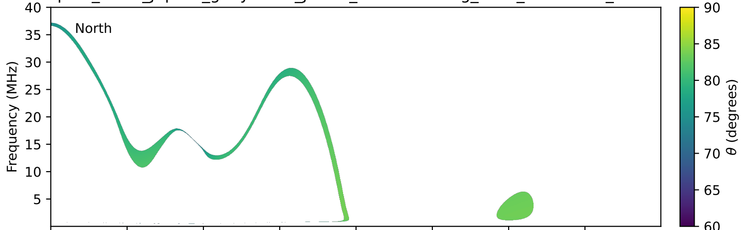
expres_earth_jupiter_ganymede_jrm33_lossc-wid1deg_3kev_20110119_v11.cdf
