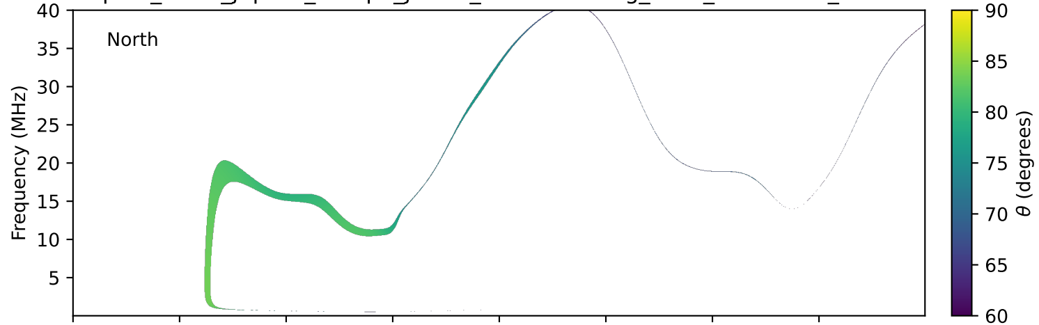
expres_earth_jupiter_europa_jrm33_lossc-wid1deg_3kev_20110127_v11.cdf
