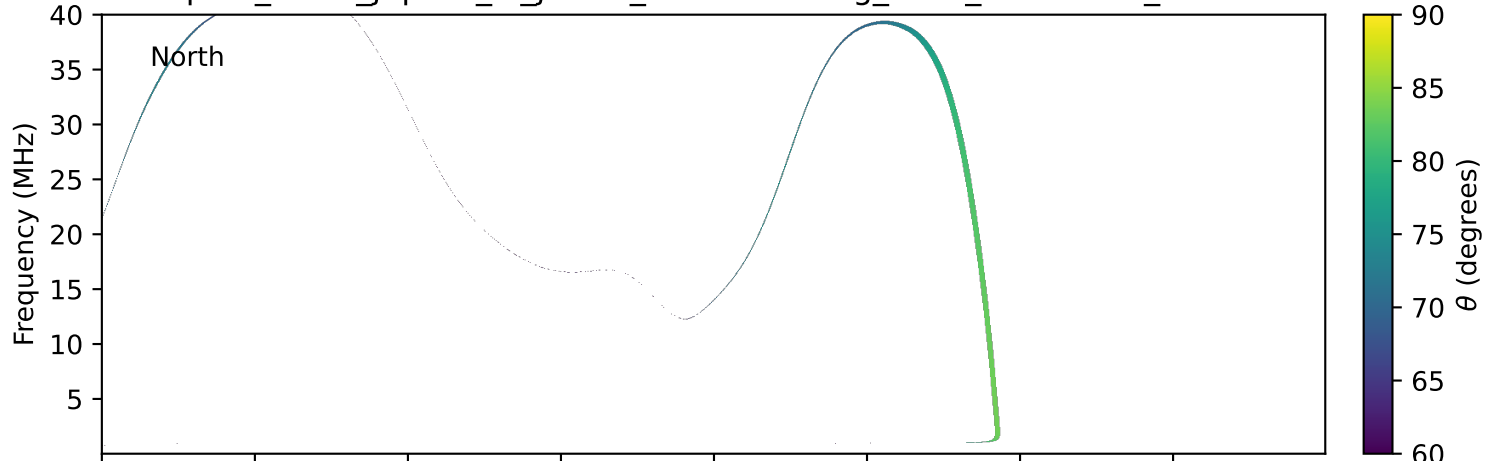
expres_earth_jupiter_io_jrm33_lossc-wid1deg_3kev_20101215_v11.cdf
