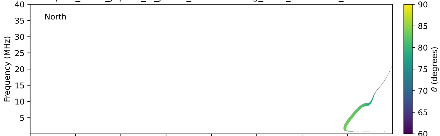
expres_earth_jupiter_io_jrm33_lossc-wid1deg_3kev_20101214_v11.cdf
