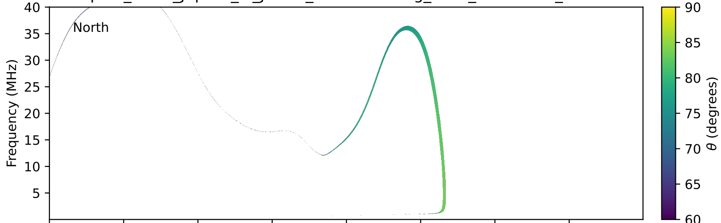
expres_earth_jupiter_io_jrm33_lossc-wid1deg_3kev_20101208_v11.cdf
