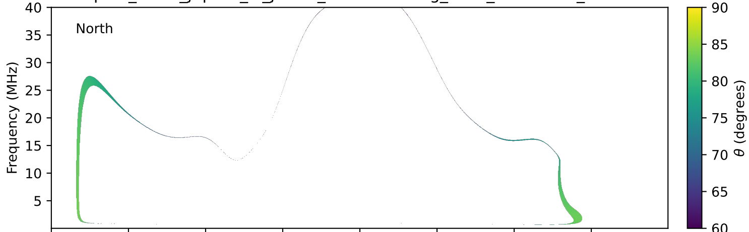
expres_earth_jupiter_io_jrm33_lossc-wid1deg_3kev_20101206_v11.cdf
