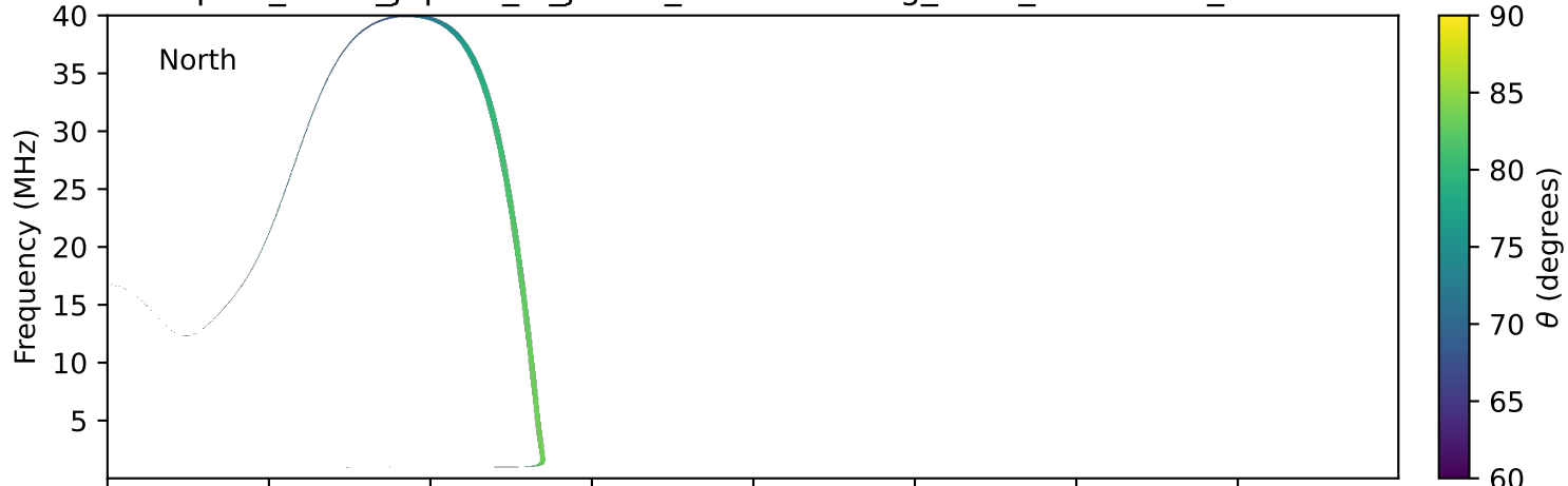
expres_earth_jupiter_io_jrm33_lossc-wid1deg_3kev_20101203_v11.cdf
