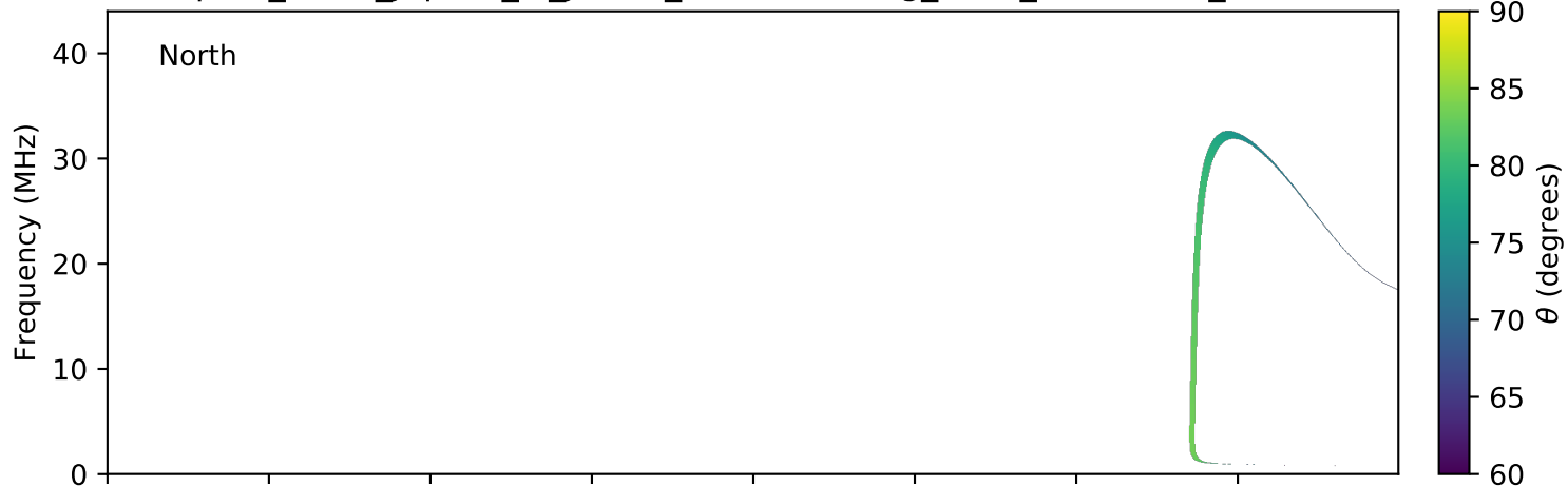
expres_earth_jupiter_io_jrm09_lossc-wid1deg_3kev_20101230_v01.cdf
