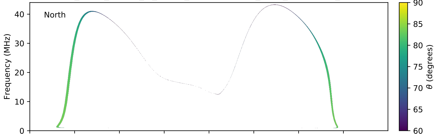
expres_earth_jupiter_io_jrm09_lossc-wid1deg_3kev_20101229_v01.cdf
