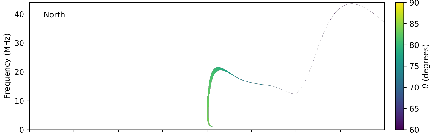
expres_earth_jupiter_io_jrm09_lossc-wid1deg_3kev_20101225_v01.cdf
