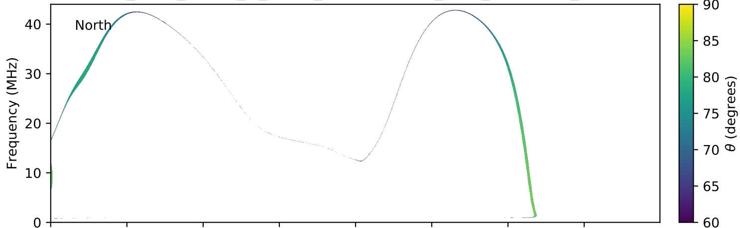
expres_earth_jupiter_io_jrm09_lossc-wid1deg_3kev_20101222_v01.cdf
