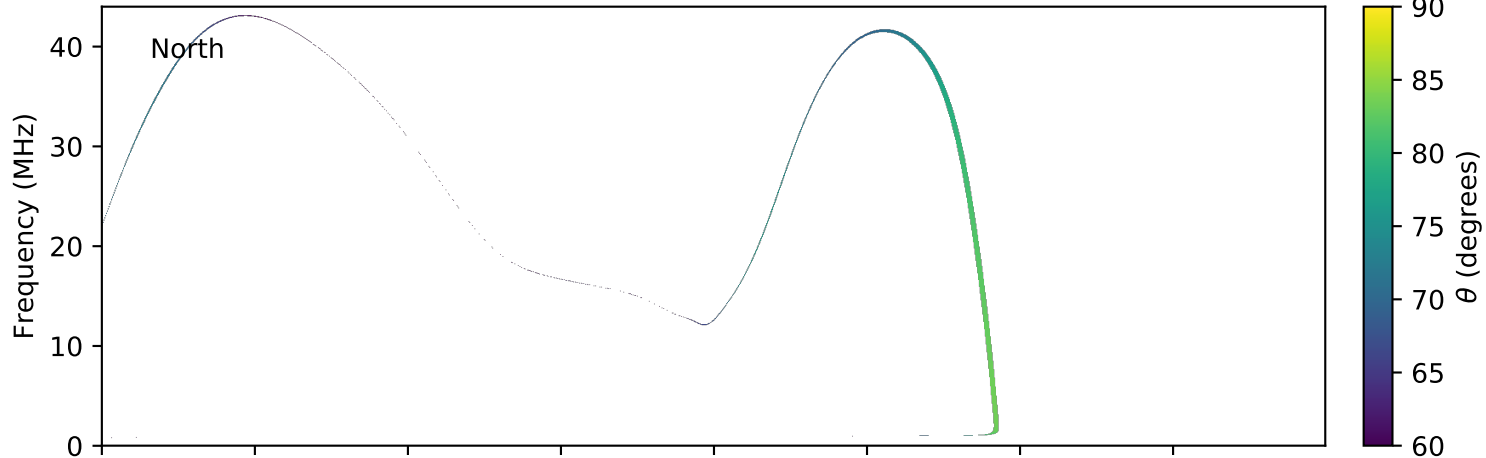
expres_earth_jupiter_io_jrm09_lossc-wid1deg_3kev_20101215_v01.cdf
