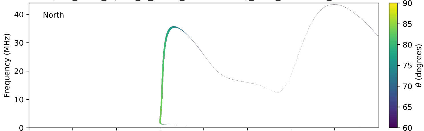
expres_earth_jupiter_io_jrm09_lossc-wid1deg_3kev_20101211_v01.cdf
