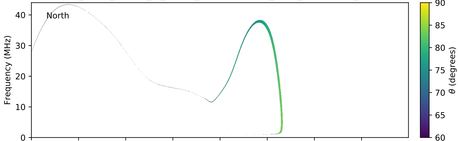
expres_earth_jupiter_io_jrm09_lossc-wid1deg_3kev_20101208_v01.cdf
