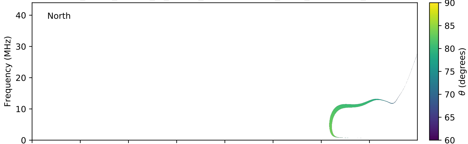
expres_earth_jupiter_io_jrm09_lossc-wid1deg_3kev_20101207_v01.cdf
