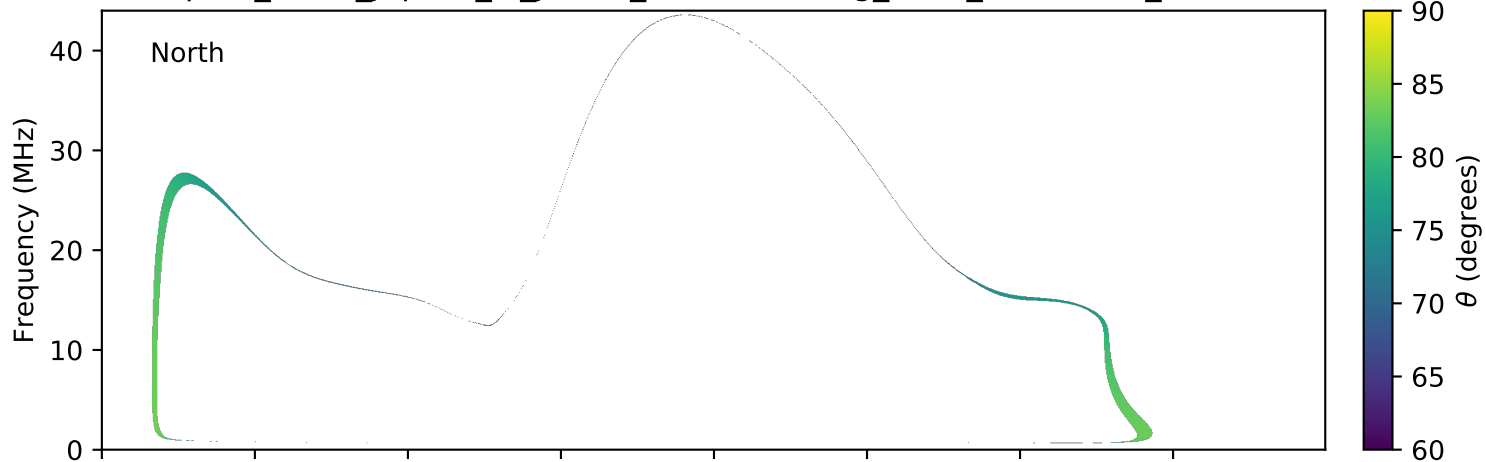
expres_earth_jupiter_io_jrm09_lossc-wid1deg_3kev_20101206_v01.cdf
