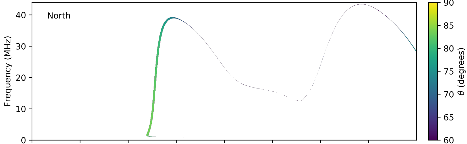
expres_earth_jupiter_io_jrm09_lossc-wid1deg_3kev_20101204_v01.cdf
