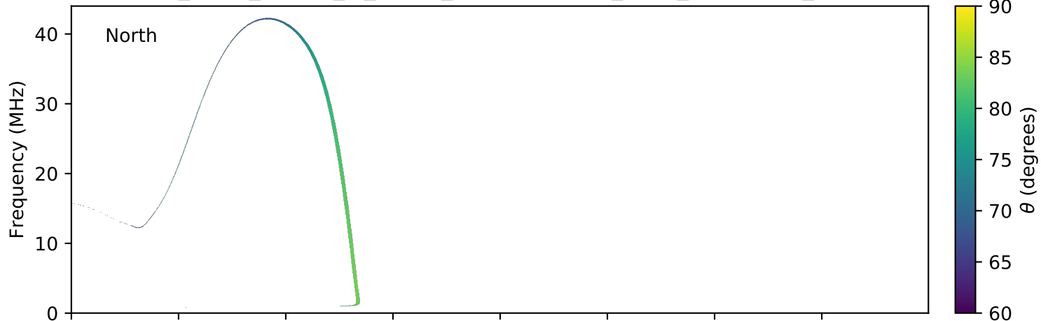
expres_earth_jupiter_io_jrm09_lossc-wid1deg_3kev_20101203_v01.cdf
