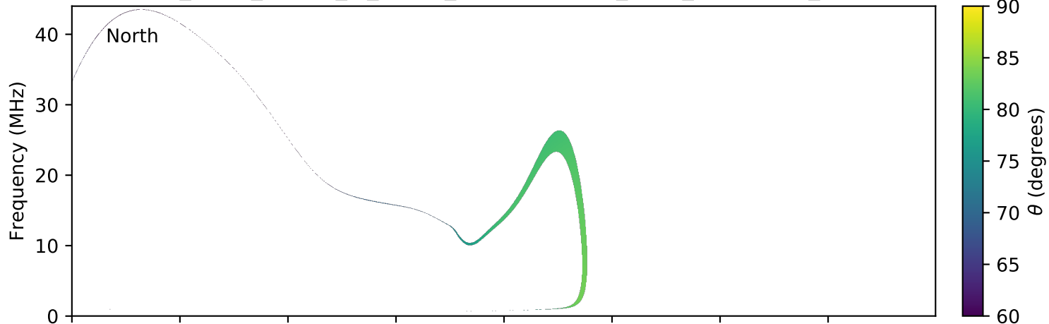
expres_earth_jupiter_io_jrm09_lossc-wid1deg_3kev_20101201_v01.cdf
