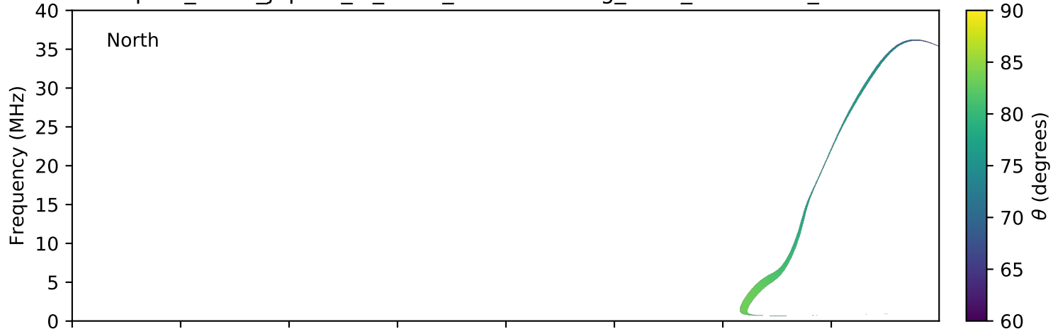
expres_earth_jupiter_io_isaac_lossc-wid1deg_3kev_20101230_v01.cdf
