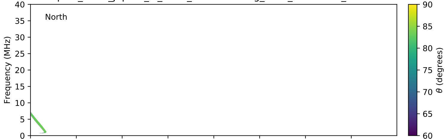
expres_earth_jupiter_io_isaac_lossc-wid1deg_3kev_20101228_v01.cdf
