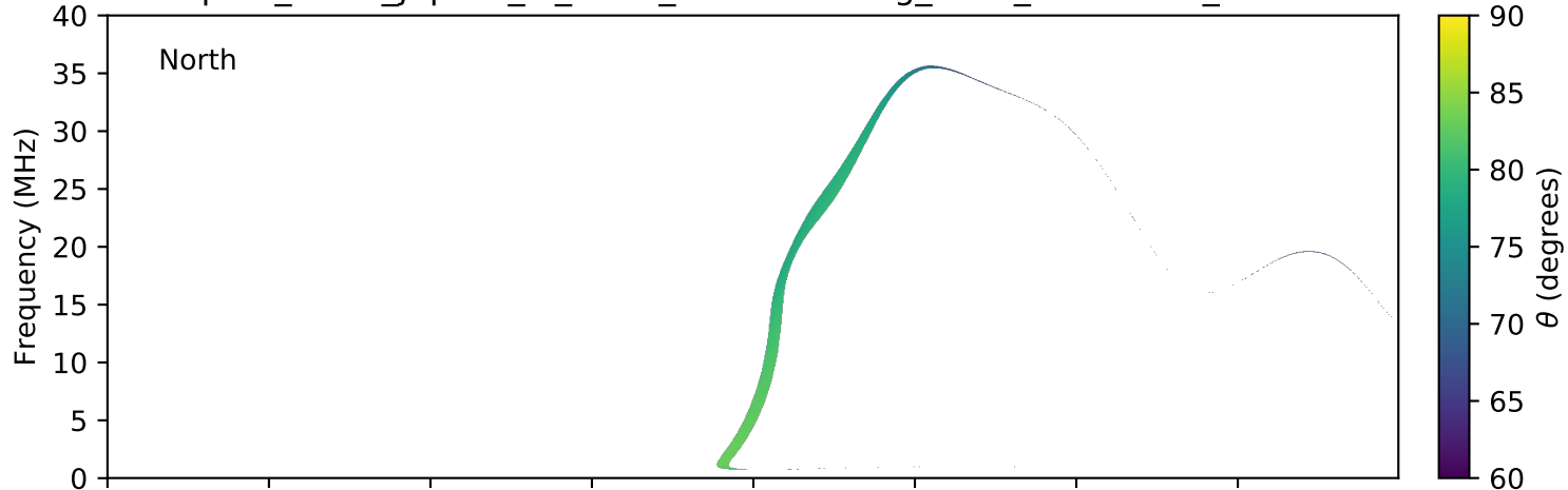
expres_earth_jupiter_io_isaac_lossc-wid1deg_3kev_20101225_v01.cdf
